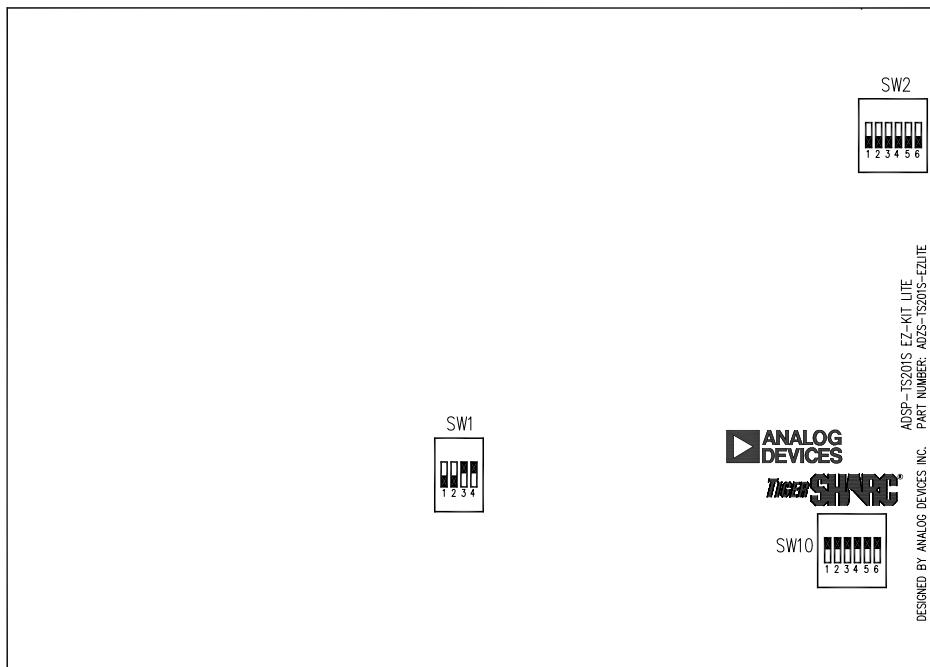
Figure 2-2. Switch Locations
