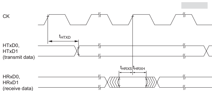
Figure 24-27 HCAN Input/Output Timing 1057 Figure amended
