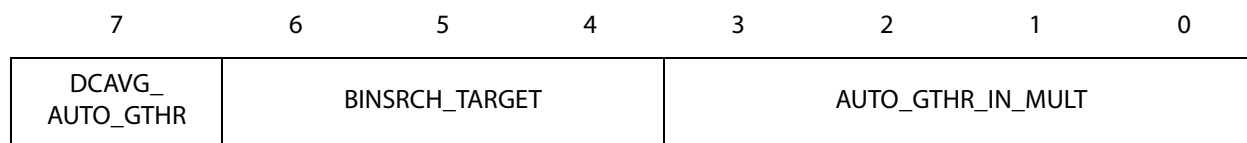
Figure 76: Calibration Configuration Register Two
