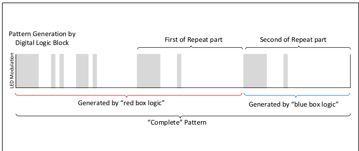
Figure 93: Pattern Generation by Logical Block
