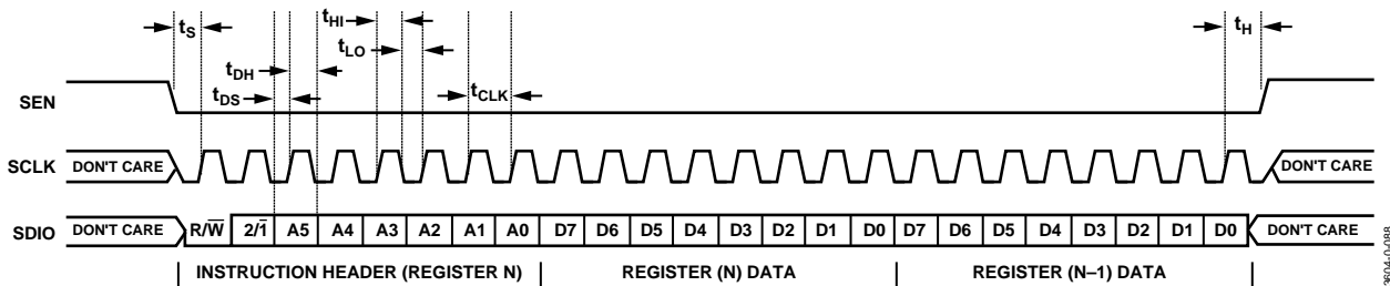
Figure 53. 2-Byte Serial Register Write in MS-First Mode
