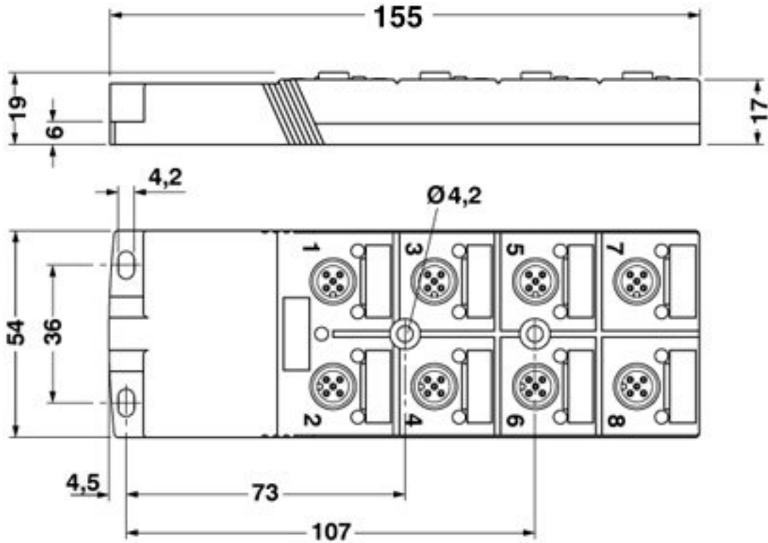
Dimensioned drawing
