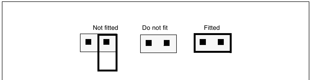
Figure 4: Jumper positions
