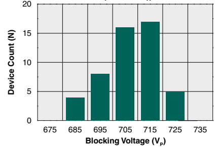
Typical Blocking Voltage Distribution (N=50, I_F=0\text{mA} , T_A=25^\circ\text{C} )
