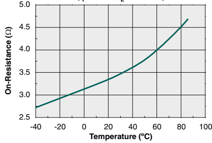
Typical On-Resistance vs. Temperature ( I_F=5mA, I_L=300mA )
