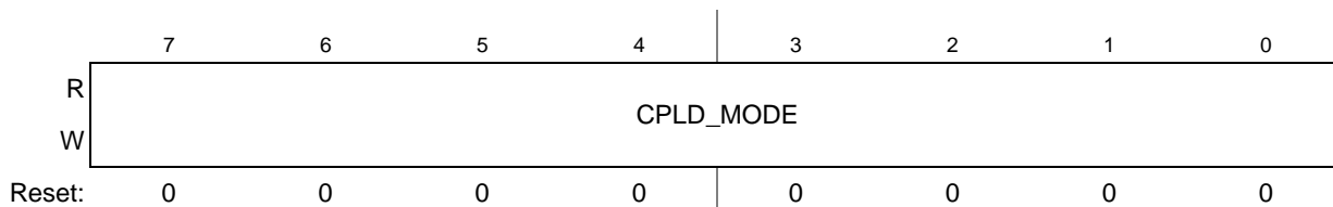
Figure 22. CPLD_MODE Register
