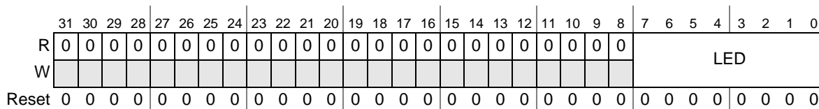
Figure 17. FPGA_7SEGMENT Register
