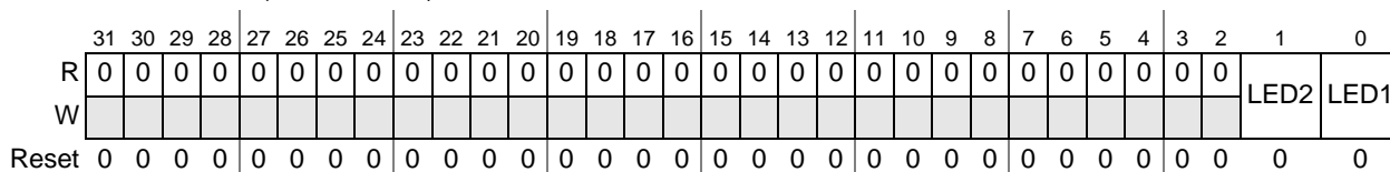
Figure 18. FPGA_LEDS Register
