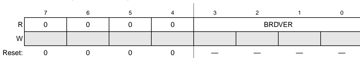
Figure 19. CPLD_VERSION Register
