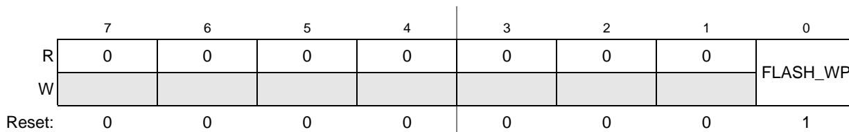
Figure 23. CPLD_FLASHCFG Register
