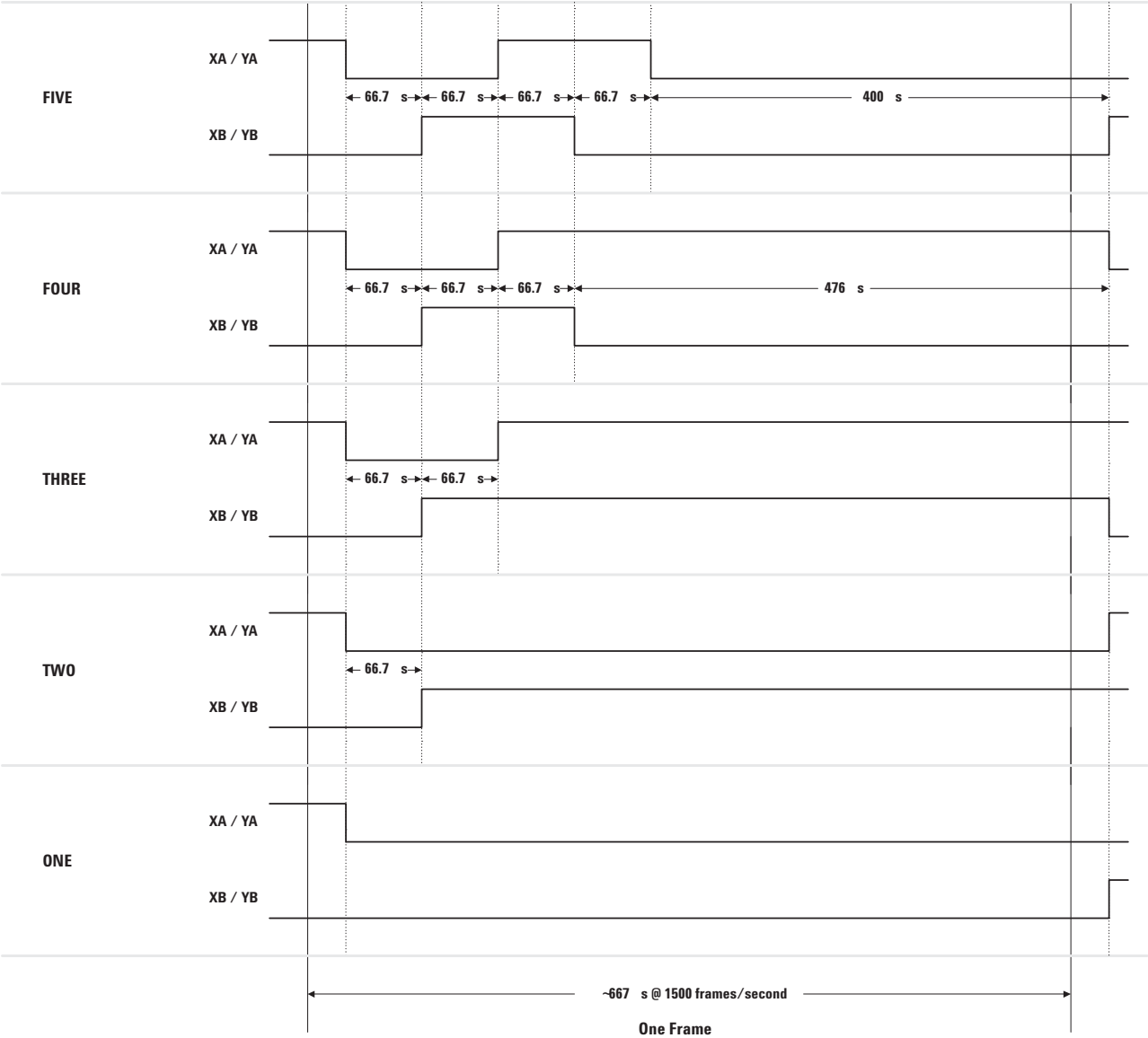
Figure 17. Quadrature states per frame (800 cpi mode).
