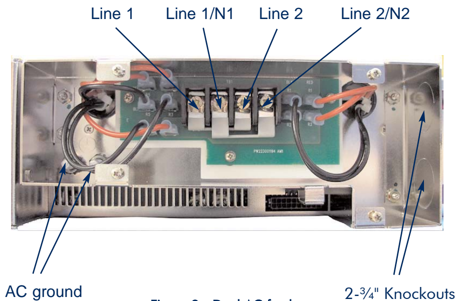
Figure 8 - Dual AC feed
