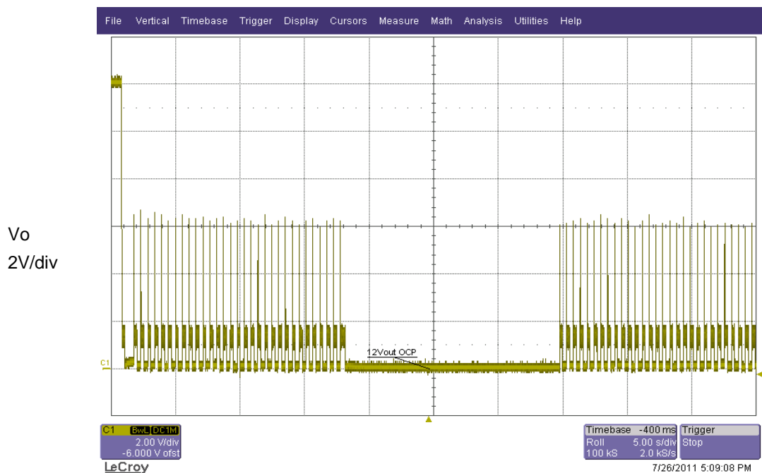
Output Voltage hiccups during OCP mode. (18s Hiccup & 16s turn off)
