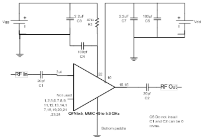
Figure 3 Evaluation Board Schematic
